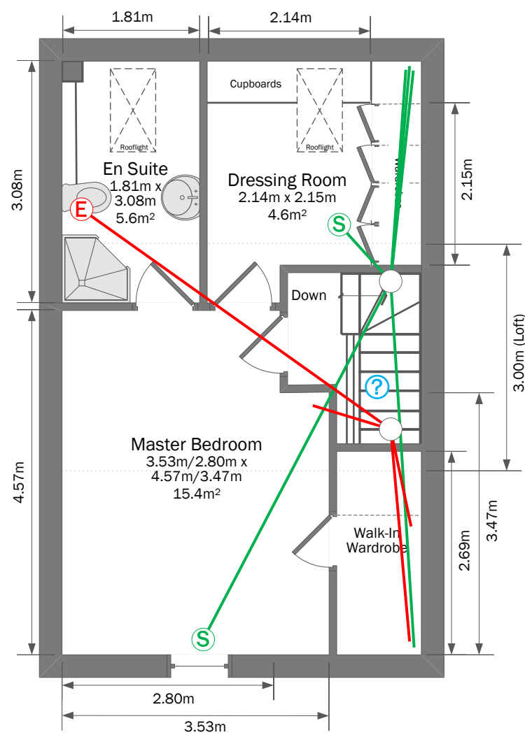
Top Floor ~37m²
